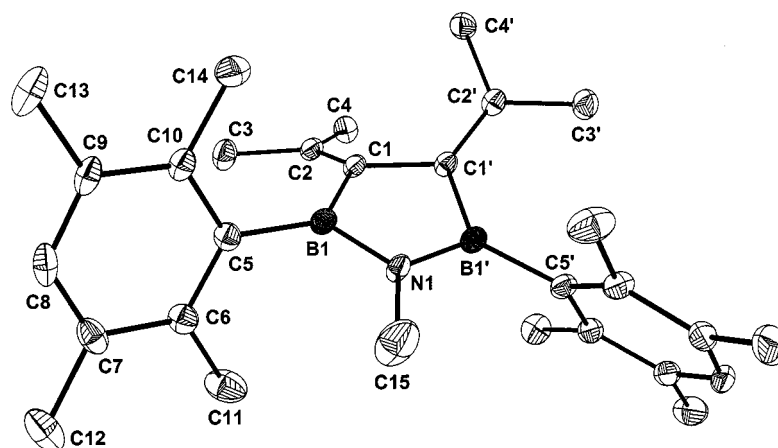
Figure 2. Molecular structure of 5b ; selected bond lengths [Å] and angles [°]: C1–C1' 1.501(6), C1–C2 1.353(4), C1–B1 1.567(5), B1–C5 1.575(5), B1–N1 1.425(4), N1–C15 1.462(7); C2–C1–C1'–C2' 51.0
