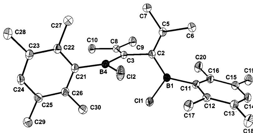
Figure 1. Molecular structure of 4c ; selected bond lengths [Å] (corresponding data for 4e in square brackets): C3–C8 1.355(3) [1.328(8)], C2–C5 1.360(3) [1.355(8)], C2–C3 1.529(3) [1.520(10), 1.510(11)], C3–B4 1.540(4) [1.574(9)], C2–B1 1.541(4) [1.560(10)], B4–Cl2 1.799(3) [B–O 1.374(8)], B1–Cl1 1.802(3) [B–O 1.377(8)], B4–C21 1.582(4) [1.589(9)], B1–C11 1.581(4) [1.590(8)].
