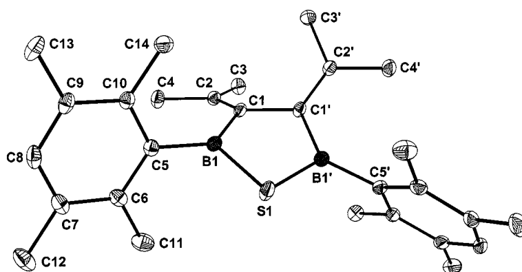
Figure 3. Molecular structure of 7 ; selected bond lengths [Å] and angles [°] (corresponding data for 6 in square brackets): C1–C1' 1.508(3) [1.500(4)], C1–C2 1.359(2) [1.358(3)], C1–B1 1.552(2) [1.571(3)], B1–C5 1.572(2) [1.570(5)], B1–S1 1.824(2) [B1–O1 1.400(2)]; C2–C1–C1'–C2' 53.8 [50.2]
